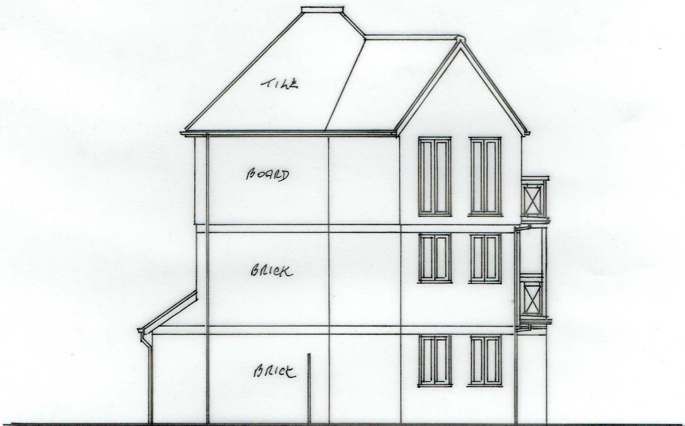
EXISTING SOUTH EAST ELEVATION (SIDE)
